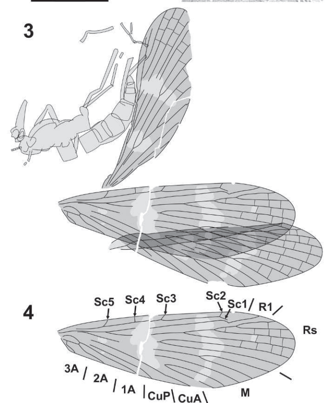
FIGURE 1— Eorpa ypsipeda n. gen. n. sp. F-1539, McAbee locality. 1, photograph; 2, closeup photograph of portion of the leg (area within square in 1) showing annular pubescence, scale=200 µm; 3, drawing of 1; 4, forewing drawing. Scale=5 mm except where noted.
