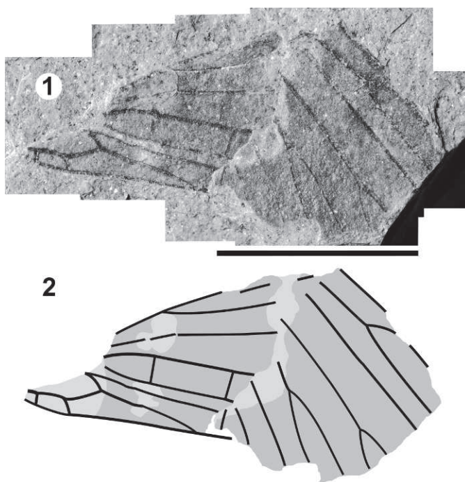
FIGURE 19—Forewing RBCM.EH2012.004.0001.001, Eorpa incertae sedis (Falkland): 1, photograph; 2, drawing. Scale=5 mm.
