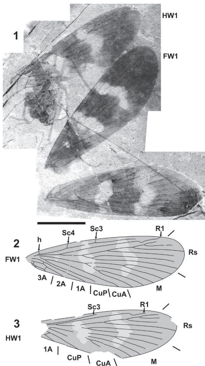
FIGURE 2— Eorpa ypsipeda n. gen. n. sp. F-1538, wings and body parts (McAbee): 1, photograph of all four wings (two overlapping); 2, drawing of forewing; 3, drawing of hind wing. Scale=5 mm.
