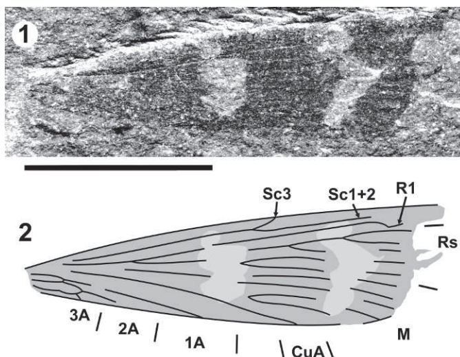
FIGURE 20—Forewing SRUI 93-14-05 (Republic exposure UWBM B4213): 1, photograph; 2, drawing. Scale=5 mm.
